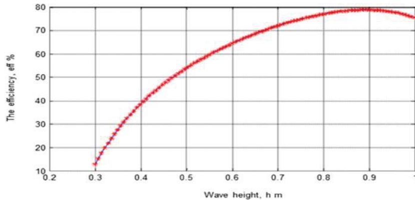
Fig. 15 Relation between wave height and the turbine efficiency
