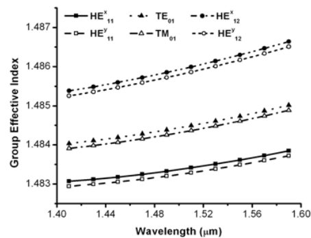
Fig. 9: Group effective index versus wavelength.
