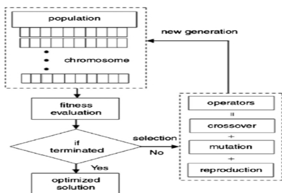
Fig. 1 Evolutionary Algorithm Flow Chart
