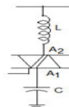
Fig. 4 Topology 1
