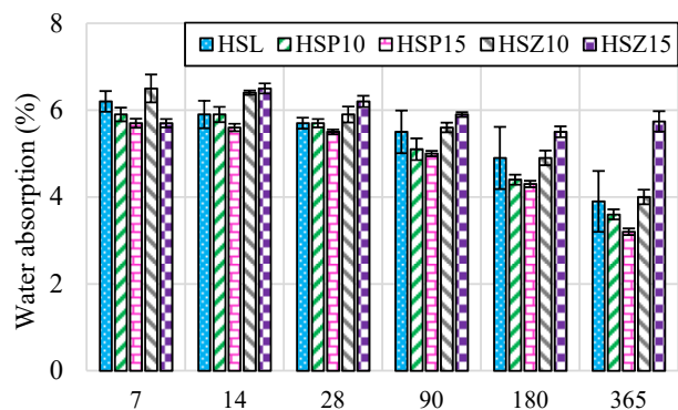
Fig. 9 Absorption after immersion (%) of studied HSSCCs
