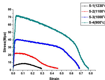
Fig. 7 True stress-true strain curves obtained from tensile tests conducted on as-cast 310S stainless steel at various temperatures
