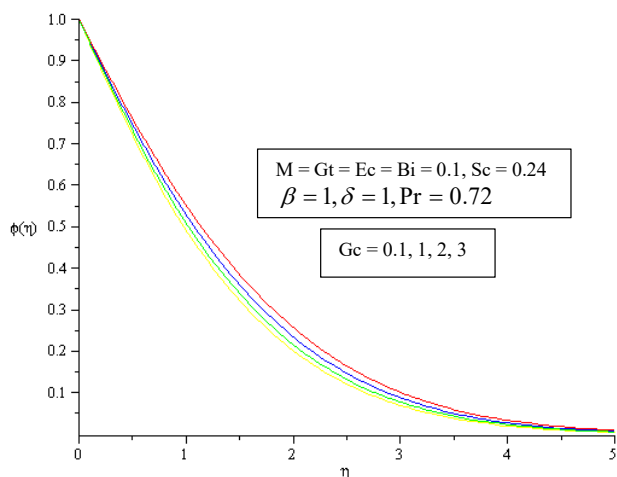
Fig. 13 Concentration Profiles with Solutal Grashof Number
