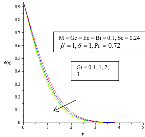
Fig. 6 Temperature Profiles with Thermal Grashof number
