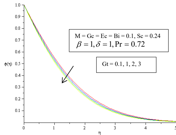
Fig. 12 Concentration Profiles with Thermal Grashof Number
