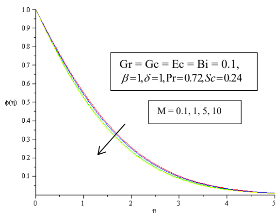
Fig. 14 Concentration Profiles with Magnetic Parameter
