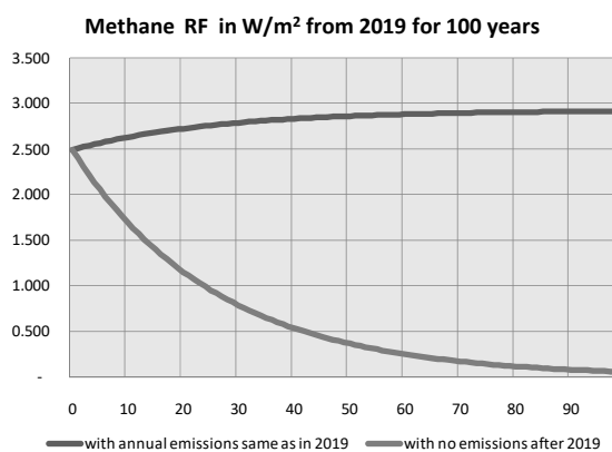
Fig. 5 Methane RF based on additional annual emissions of 2019 (dark line) and no additional emissions (grey line)
