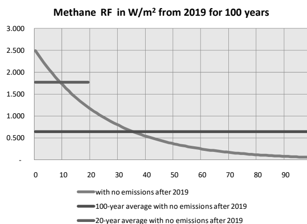
Fig. 3 Methane RF as a function of time after initial emission
