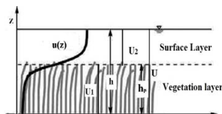
Fig. 1 Velocity profile within and above vegetation
