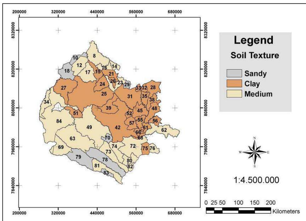
Fig. 7 Map of soil texture to southwest Goiás
