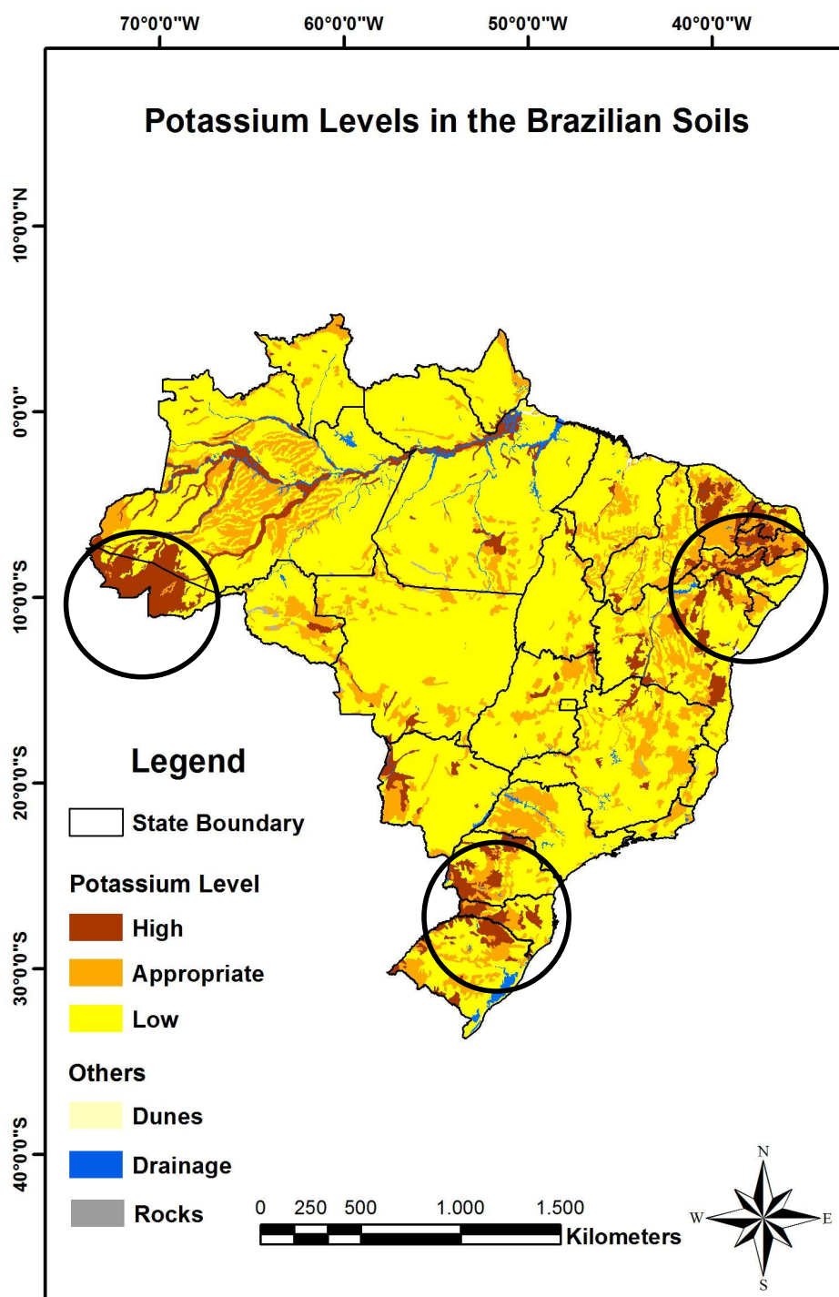
Fig. 4 Map of potassium level in brazilian soils
