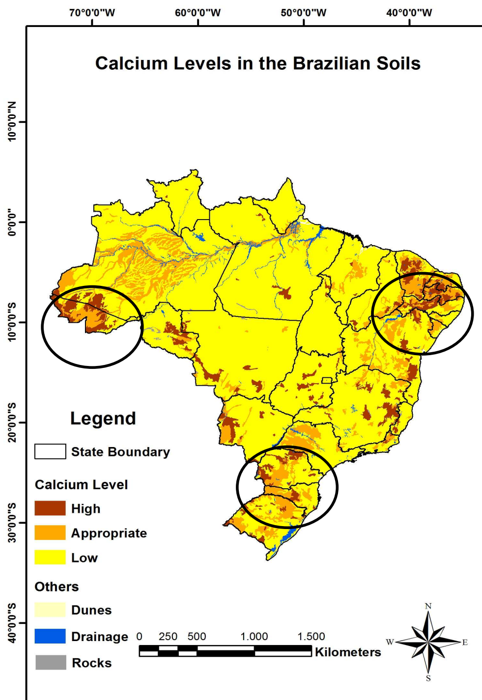
Fig. 6 Map of calcium level in brazilian soils
