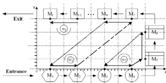
Fig 4 U shaped Assembly Line
