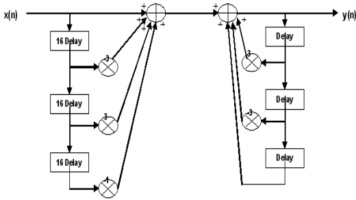
Fig. 7 CIC filter in polynomial representation
