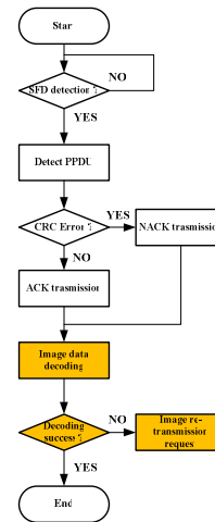
(b) Receiver
