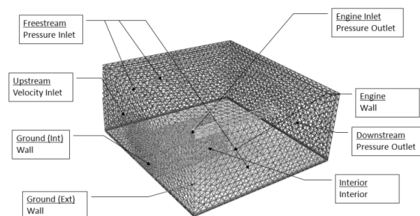
Fig. 5 Boundary Conditions
