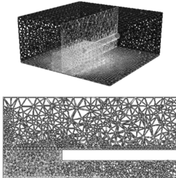
Fig. 4 Flow Model
