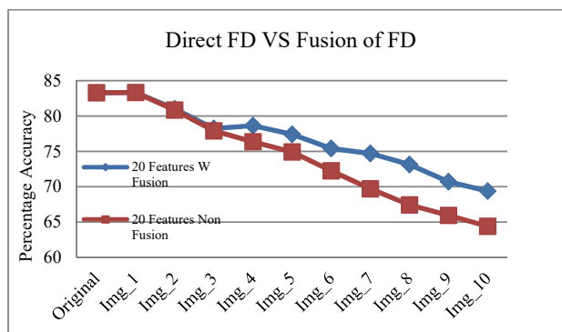
Fig. 4 Classification accuracy between extracting features from FD image and proposed Fusion of images
