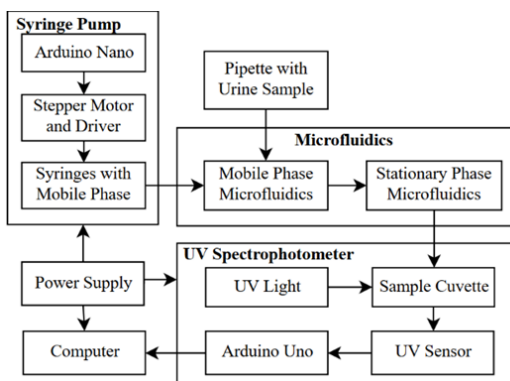
Fig. 2 Hardware Block Diagram
