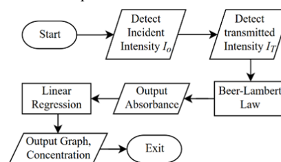
Fig. 4 Quantification of Urine Albumin Flowchart
