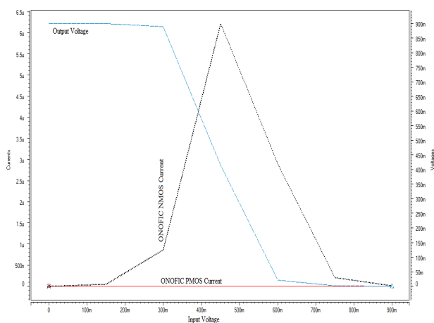
Fig. 5 ONOFIC transistors current
