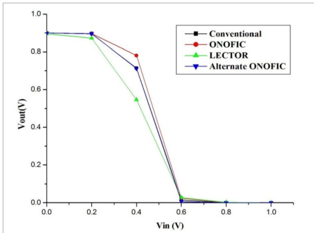
Fig. 4 DC Characteristic of CMOS inverter
