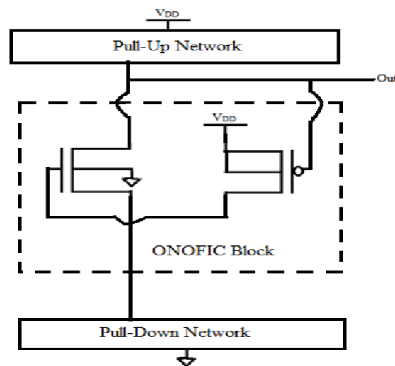
Fig. 2 ONOFIC Schematic
