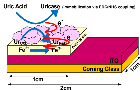
Fig. 2 Schematic of the prepared uricase/PANI/ITO/glass bioelectrode
