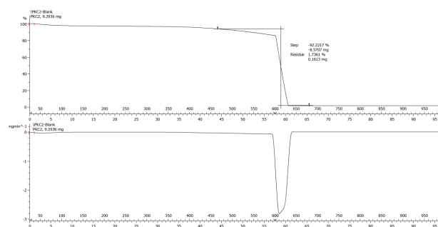
Fig. 3 TGA curve of palm kernel shell
