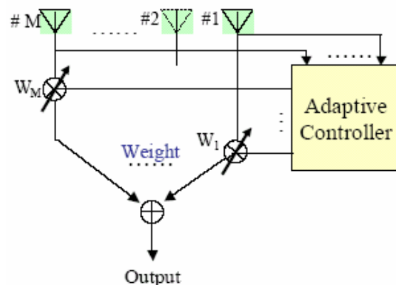
Fig. 3 Diagram of Basic Adaptive Antenna System
