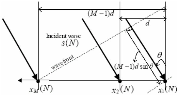
Fig. 4 Uniform Linear Array of M -Element
