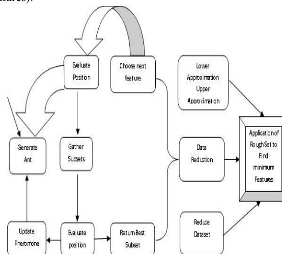
Fig. 1 Proposed Hybridized Model using ACO and RST (Rough ACO)
