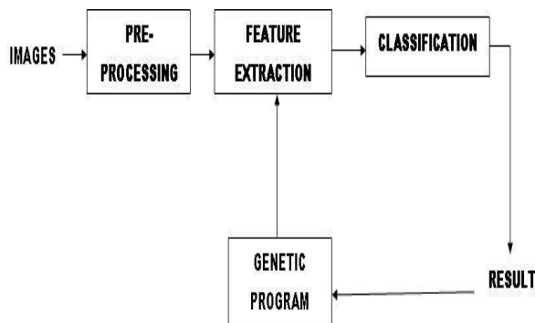
Fig. 2 Feature Extraction Discovery using Genetic Programming
