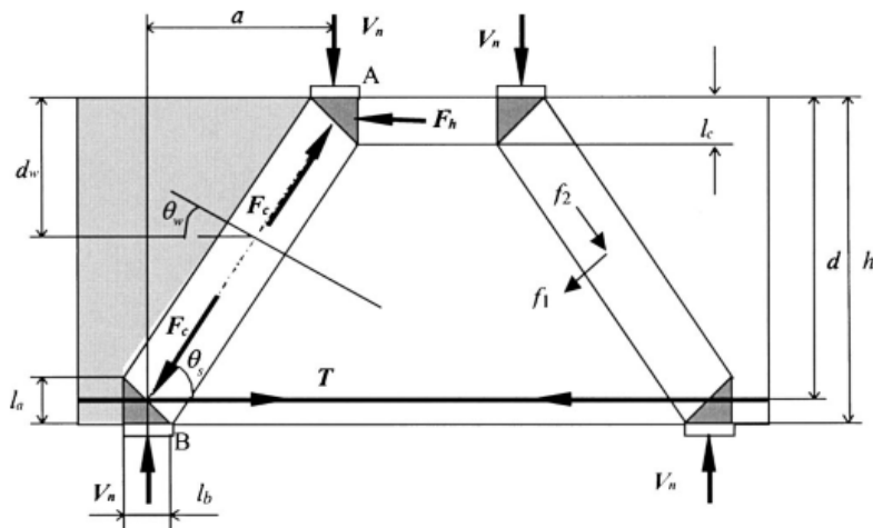
Fig. 12 Schematic shape of STM method
