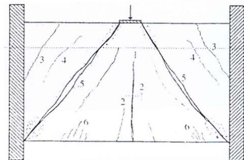
Fig. 10 Schematic shape of shear failure mode
