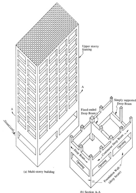
Fig. 2 Continuous deep beams supported on concrete columns
