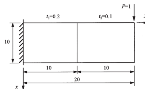
Fig. 5 Schematic of cantilever deep beam
