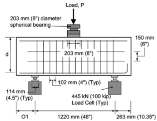
Fig. 3 Schematic of simply supported deep beam
