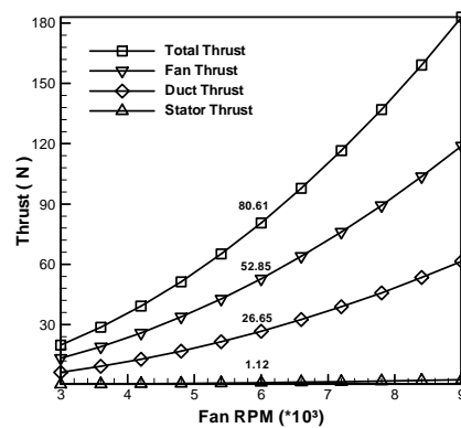
Fig. 7 The thrust components of the ducted fan system with stator
