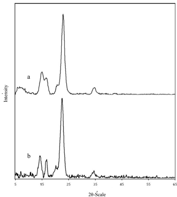
Fig. 5 XRD graphs of (a) cellulose, (b) BC.
