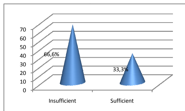
Fig. 1 Sufficiency situations of distributed cattle
