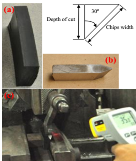
Fig. 1 (a) Experimental HDPE sample, (b) HSS cutting tool and (c) Experimental shaper machine
