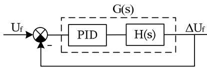
Fig. 6 The diagram of the closed-loop system with a PID regulator
