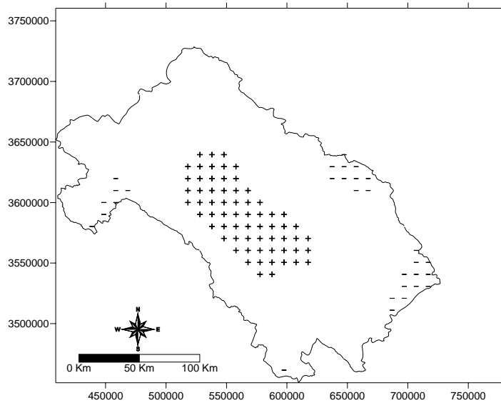
Fig.6 Temperature changes in Zayanderood watershed
