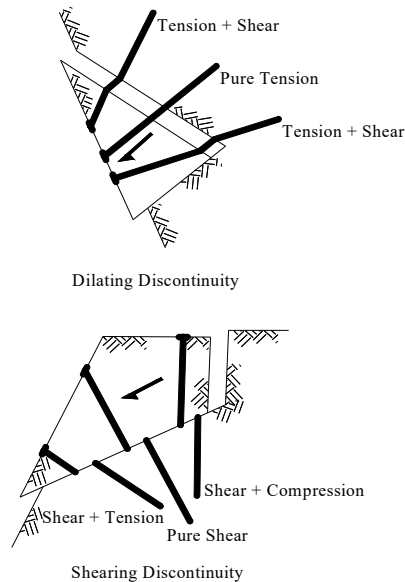
Fig. 2 Reinforcement behavior at discontinuity [2], [20]
