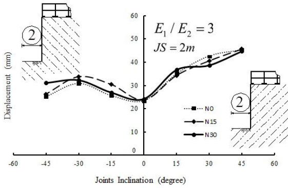
Fig. 9 Effect of joints inclination on lateral bulging where anisotropy equals to 3
