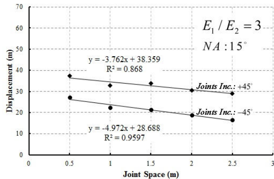
Fig. 13 Effect of joints inclination on MS
