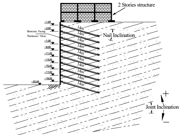
Fig. 3 Schematic of FE model and dimensions of RNW
