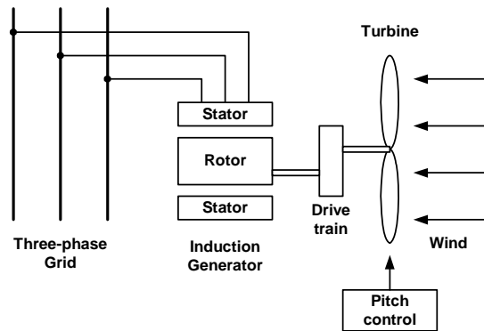
Fig. 1 Block diagram of wind turbine induction generator
