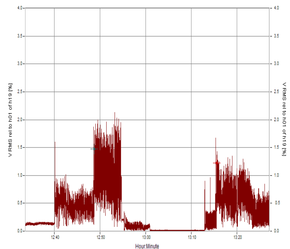
Fig. 9 19 th harmonics time variations
