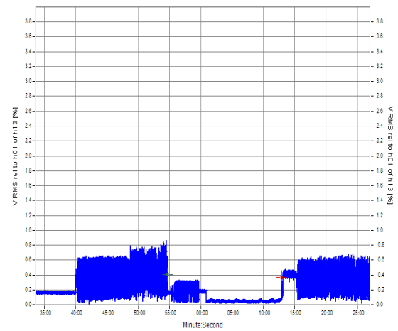
Fig. 8 (b) 13 th harmonics
