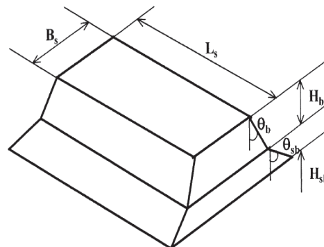
Fig. 1 The trapezoidal shape of the stress distribution under the rail sleeper of both divisions [4]
