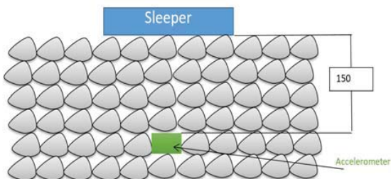
Fig. 8 Position of the accelerometer under the sleeper
