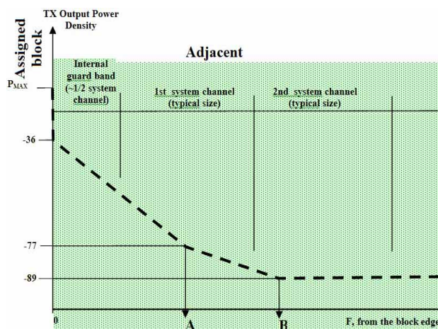
Fig. 6 Suppression mask of 3.5MHz bandwidth for FWA
