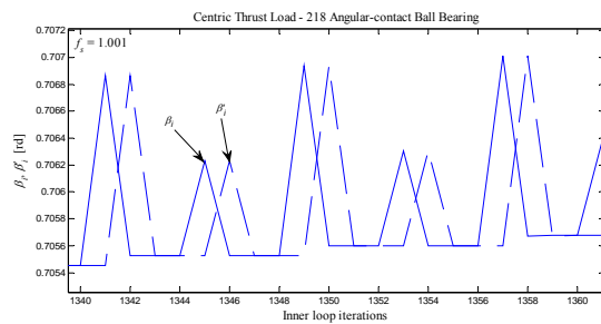
Fig. 18 Convergence procedure of the contact angle \beta_i and the inner loop auxiliary variable \beta_i' (detail)
