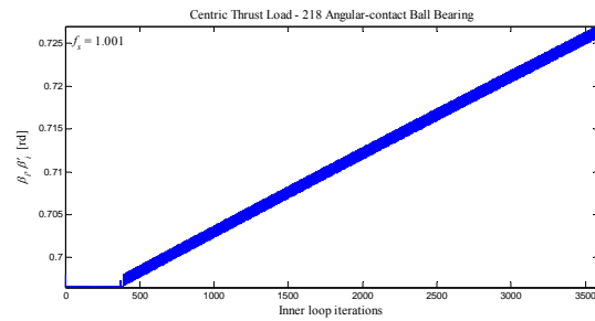
Fig. 17 Convergence procedure of the contact angle \beta_i and the inner loop auxiliary variable \beta_i'
