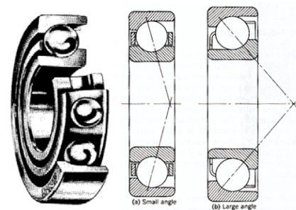
Fig. 1 Angular-contact ball bearing
