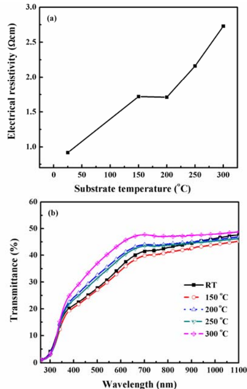
Fig. 2 (a) Electrical resistivity and (b) optical transmittance spectra of p\text{-Ni}_{1-x}\text{O}:\text{Li} thin films (with glass substrate) deposited at various substrate temperatures
