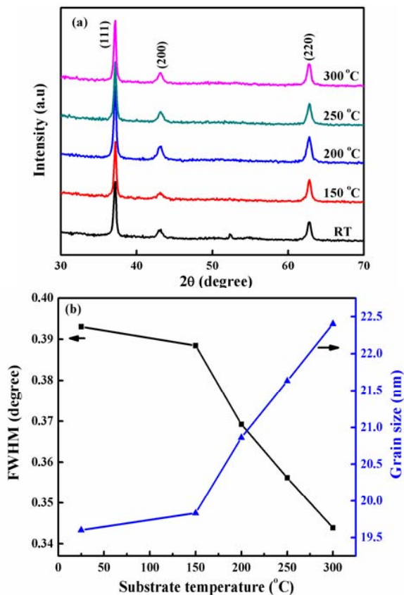
Fig. 1 (a) X-ray diffraction \theta - 2\theta scan data and (b) FWHM and grain size of NiO (111) diffraction peak for p\text{-Ni}_{1-x}\text{O}:\text{Li} thin films prepared at various substrate temperatures
