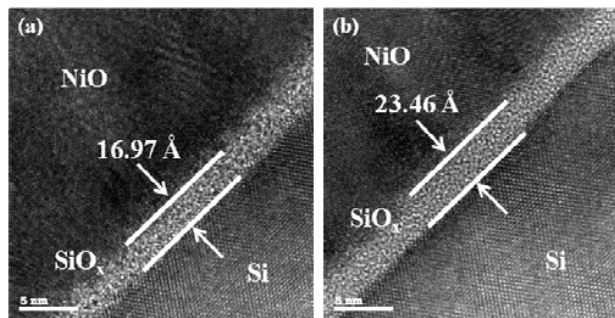
Fig. 4 Cross-sectional TEM micrographs of \text{p-Ni}_{1-x}\text{O:Li/n-Si} HJSC prepared at substrate temperatures of (a) RT (b) 300^\circ\text{C}
