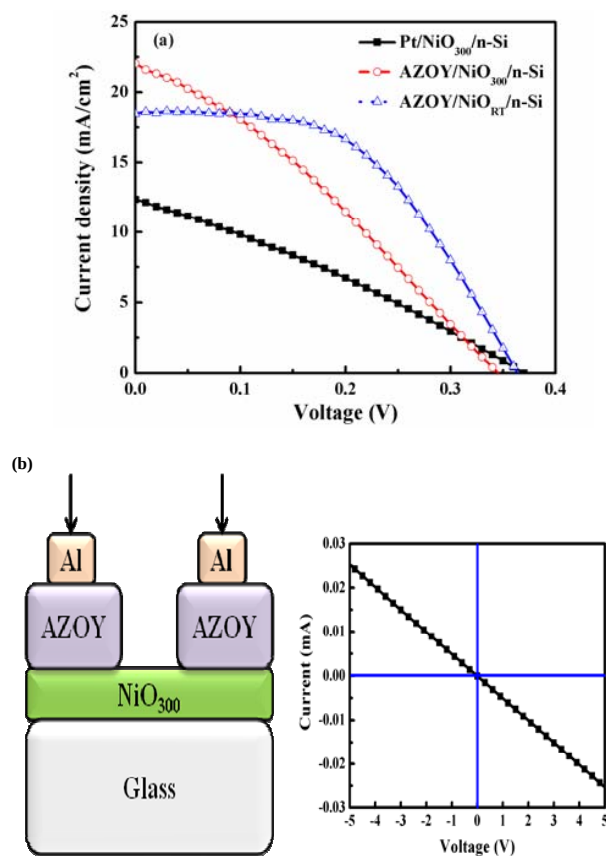
Fig. 3 (a) J - V characteristics of cells measured under 100 \text{ mW}/\text{cm}^2 illumination (AM1.5 condition) for Pt/ \text{NiO}_{300} /n-Si, Al/AZOY/ \text{NiO}_{300} /n-Si, Al/AZOY/ \text{NiO}_{\text{RT}} /n-Si, respectively. (b) I - V characteristics of Al/AZOY/ \text{NiO}_{300} HJ
