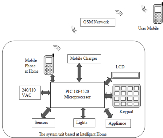
Fig. 1 Architecture of Intelligent Home system
