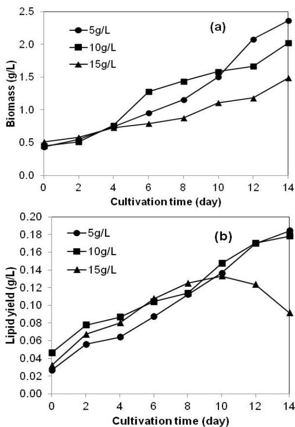
Fig. 2 Biomass concentration (a), lipid yield (b) of Chlorella sp. KKU-S2 on Bristol medium supplemented with different nitrogen concentration under photoautotrophic cultivation
