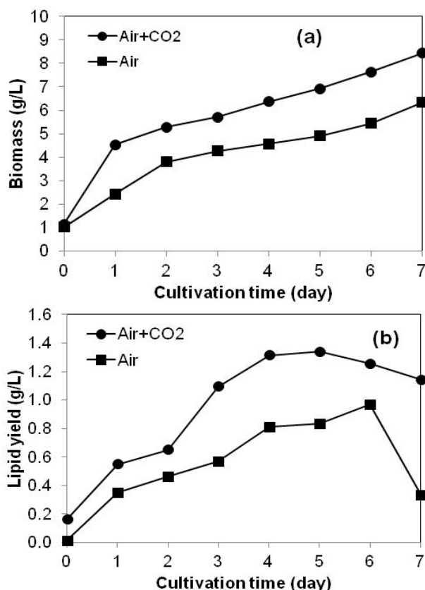
Fig. 5 Biomass (a) and lipid yield (b) of Chlorella sp. KKU-S2 under photoautotrophic cultivation by using CO_2 coupled with CO_2 emissions from yeast fermentation (Air + CO_2 ) and CO_2 from air (Air)
