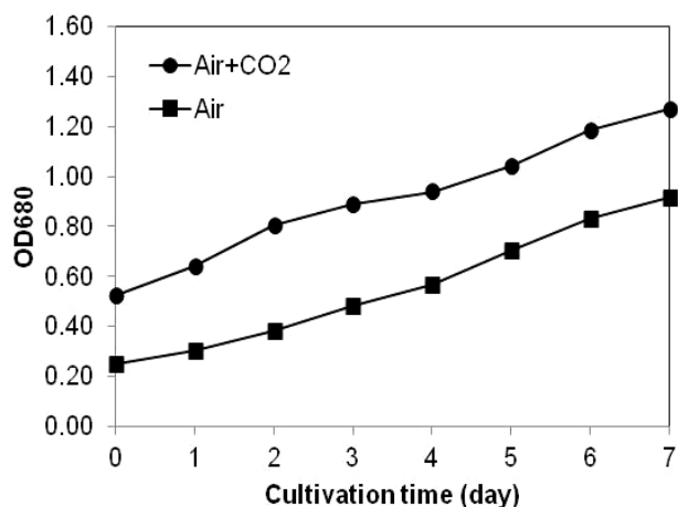
Fig. 4 Optical density ( OD_{680} ) of Chlorella sp. KKU-S2 under photoautotrophic cultivation by using CO_2 coupled with CO_2 emissions from yeast fermentation (Air + CO_2 ) and CO_2 from air (Air)
