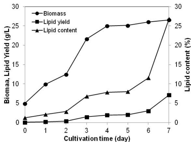
Fig. 3 Time course of cell growth of T. maleeae Y30 on LA medium using glucose as carbon source, cultivated at ambient temperature for 7 days
