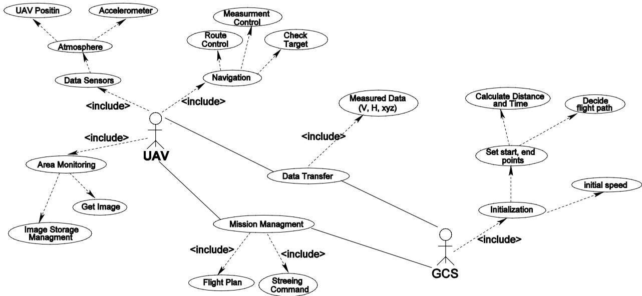
Fig. 4 UAV System use-case diagram of Functional Requirements
