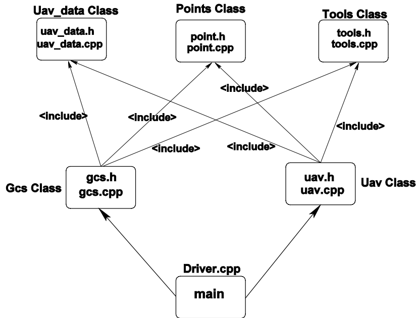
Fig. 13 UAV System Program Structure
