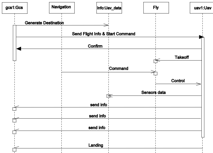
Fig. 14 UAV System Sequence Diagram
