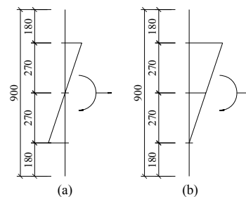
Fig. 7 Calculation diagram of bound force (Units: mm)
