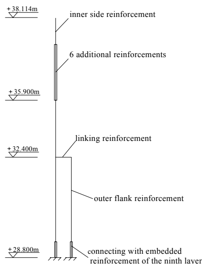
Fig.1 Single steel mesh model
