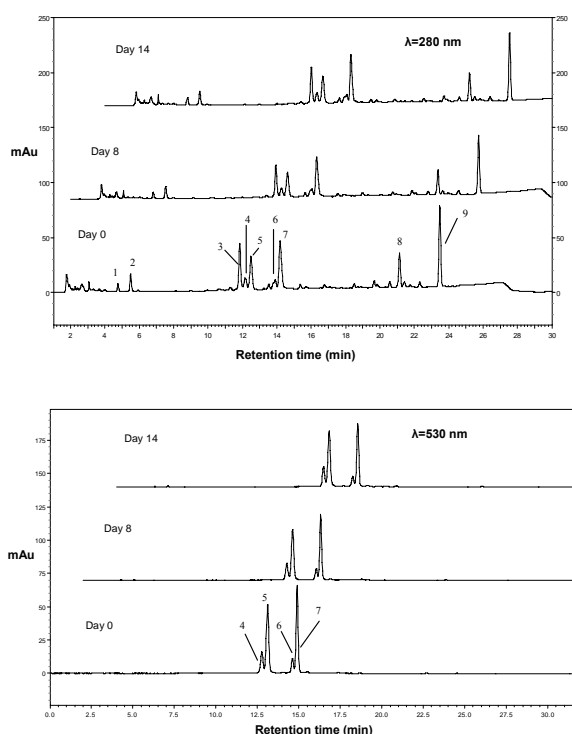
Fig. 2 HPLC chromatograms at 280 and 530 nm for a smoothie containing 750 mg polyphenols and 7.5 g fibre during storage at 4°C for 14 days. Peak 1: Unknown; Peak 2: Catechin derivative; Peak 3: Chlorogenic acid; Peak 4: Delphinidin-3- O -rutinoside; Peak 5: Delphinidin-3- O -glucoside; Peak 6: Cyanidin-3- O -rutinoside; Peak 7: Cyanidin-3- O -glucoside; Peak 8: Phloridzin; Peak 9: Quercetin
