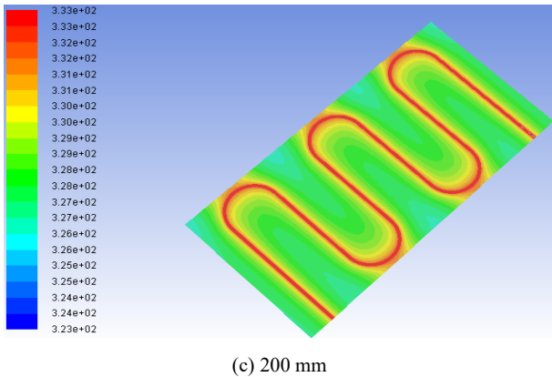
Fig. 3 Mid-section concrete slab temperature distribution
