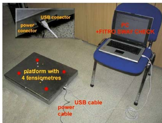
Fig. 1 System for stabilometric measurement
