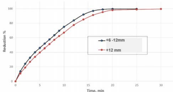
Fig. 6 The reduction curves for different pellet size of iron ore B
