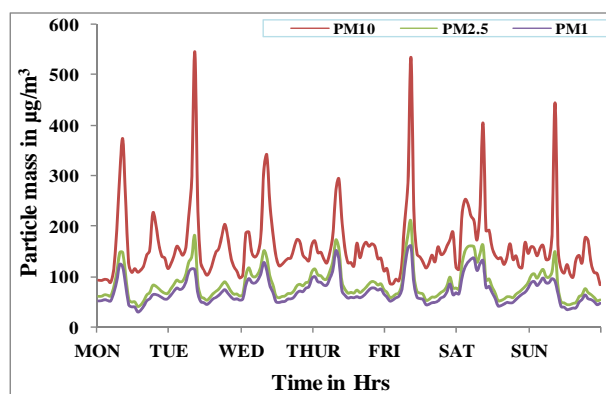
Fig. 2 Hourly variations of coarse and fine particle matters at the study area
