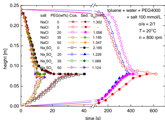
Fig. 7 Comparison coalescence and sedimentation curve of o/a = 2/1 at different concentrations of PEG4000 and 100 mmol/L NaCl and \text{Na}_2\text{SO}_4
