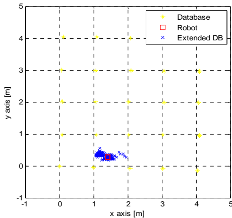
Fig. 7 Output of extended DB
