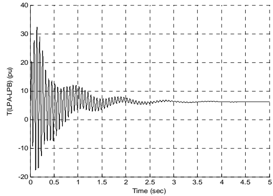
Fig. 5 Variation of shaft torsional torque (LPA-LPB) with CBVLC
