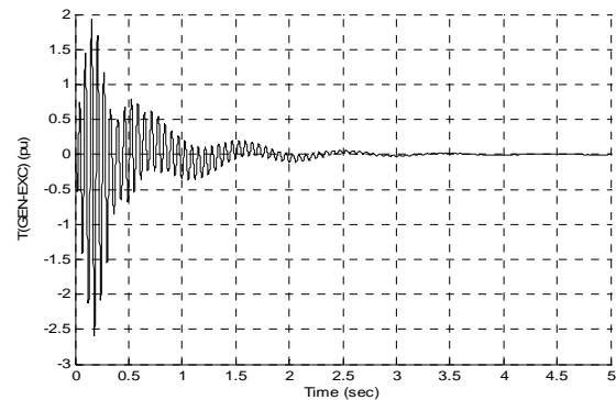
Fig. 7 Variation of shaft torsional torque (GEN-EXC) with CBVLC
