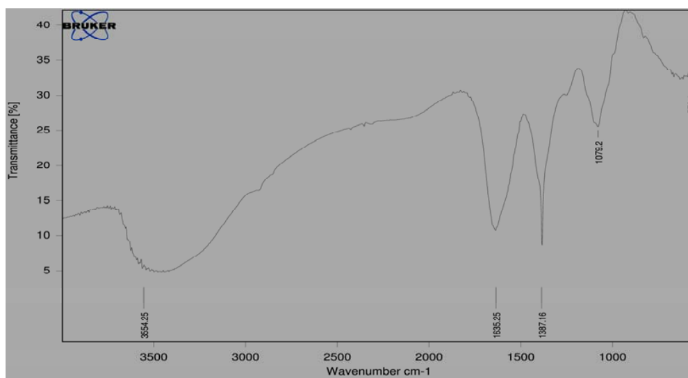
Fig. 5 FTIR spectrum of BSSNP
