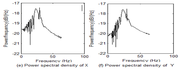
Fig. 5 (A) Dynamic response, no torsional flexibility, rub, crack but axial force, \Delta K_{\xi}/K_b=0 , \Psi=0 , P=2kN : (a) Vertical deflection of uncracked shaft; (b) Rotor response orbit; (c) X-Lateral frequency; (d) Y-lateral frequency; (e) X-Lateral power spectra; (f) Y-Lateral power spectra
