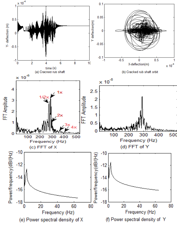
Fig. 7 (B) Rotor system response of the lateral-rotor model without torsional flexibility, with rotor-to-stator rub, small axial force and crack, \Delta K_{\xi}/K_b=0.9542, \Delta=2.65 \times 10^{-7}m P=2000N (a) Vertical cracked shaft deflection (b) Rotor response orbit, (c) X-Lateral frequency signal (d) Y-Lateral frequency signal (e) X-Lateral power spectral density (f) Y-Lateral power spectral density.
