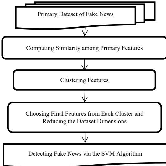
Fig. 1 Flowchart of the Proposed Method
